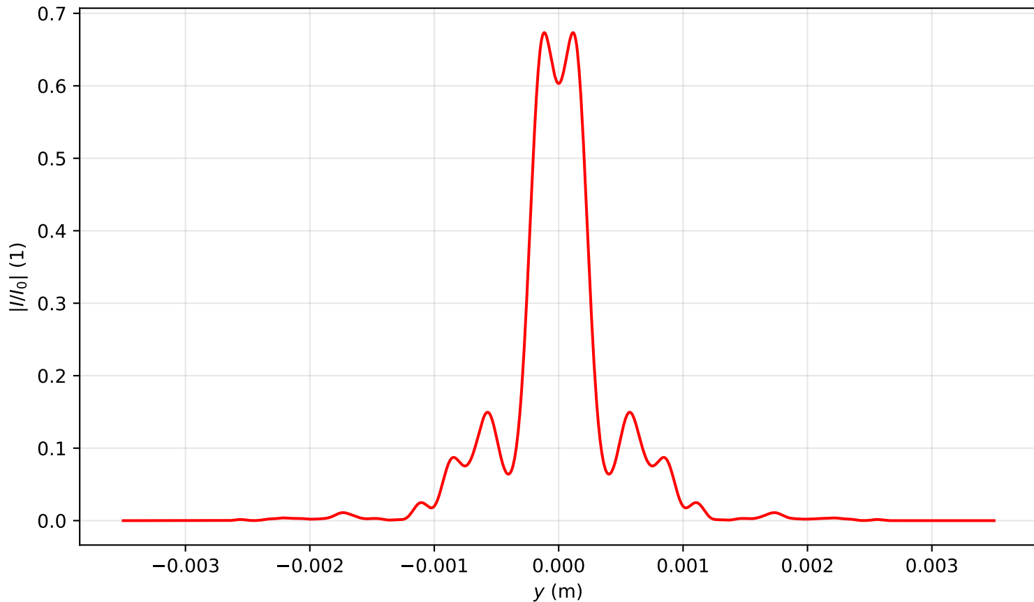
Intensity profile I(x=0, y, z=1.433)/I_0 , \text{Pin}=7.5\text{Pcr} , artificial time
